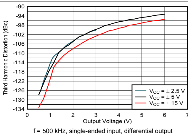
Figure 6-12. Third-Harmonic Distortion vs Output Voltage
