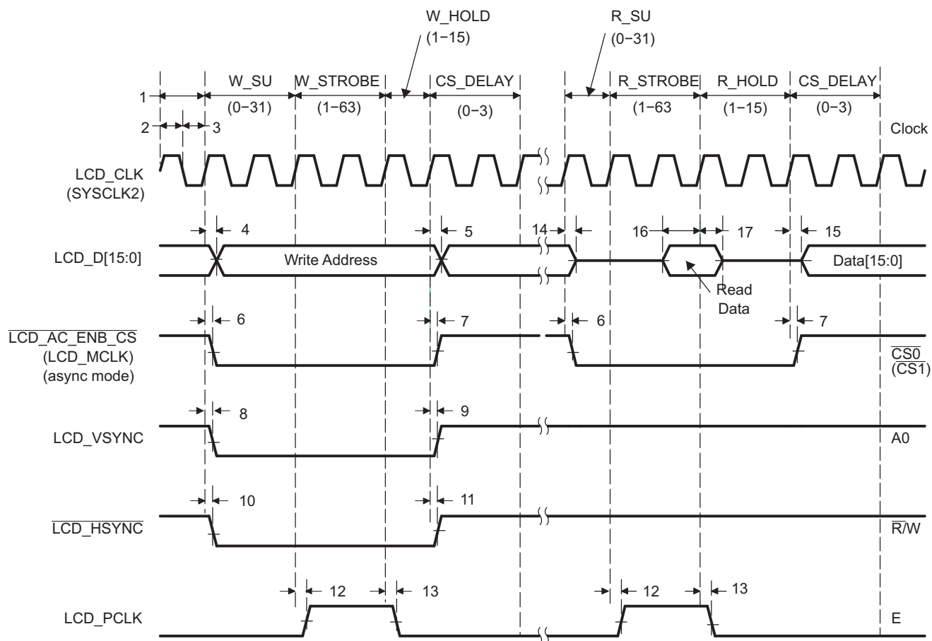
Figure 5-58. Micro-Interface Graphic Display 6800 Read
