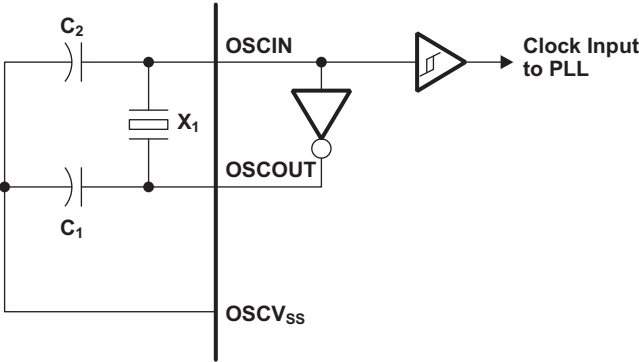
Figure 5-7. On-Chip Oscillator
