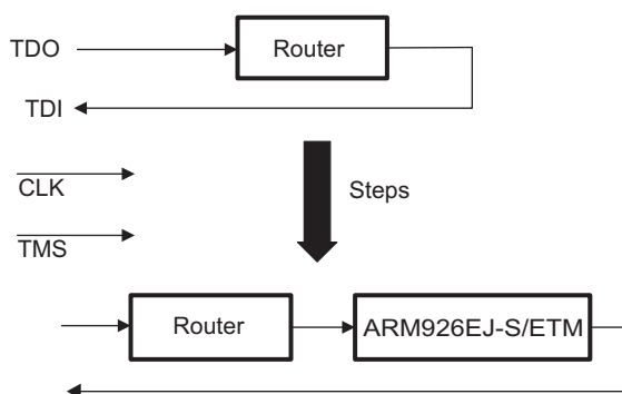
Figure 6-63. Adding ARM926EJ-S to the scan chain
