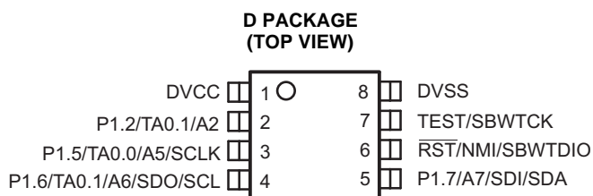
Figure 1. Device Pinout
