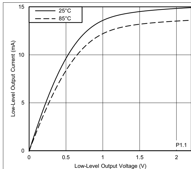
V_{CC} = 2.2\text{ V} Figure 5-9. Typical Low-Level Output Current vs Low-Level Output Voltage
