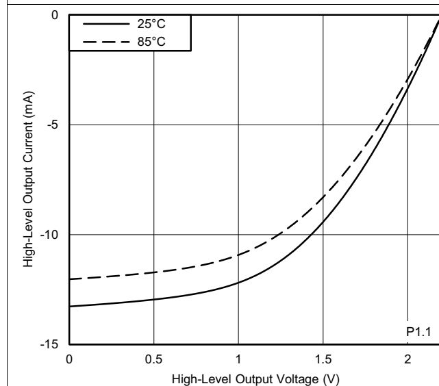
V_{CC} = 2.2\text{ V} Figure 5-11. Typical High-Level Output Current vs High-Level Output Voltage
