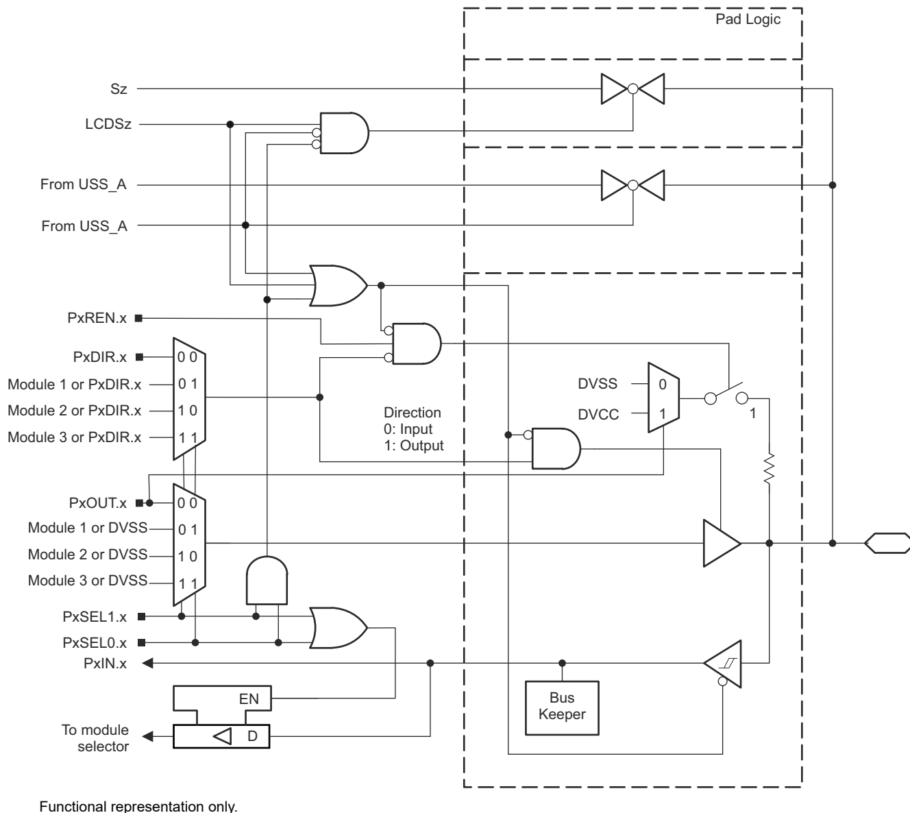
Figure 9-24. Port P7 (P7.0) Diagram
