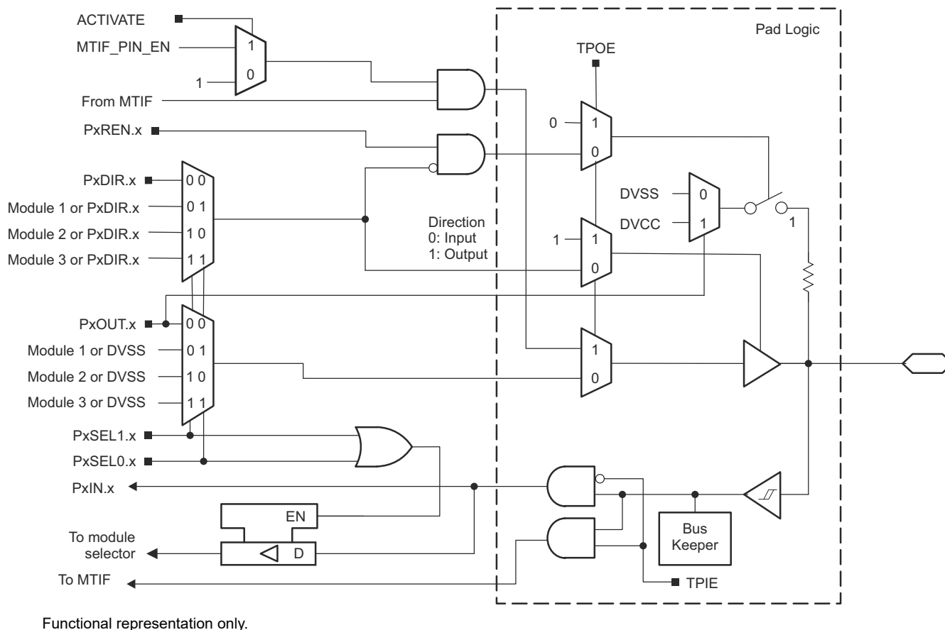
Figure 9-11. Port P3 (P3.1) Diagram
