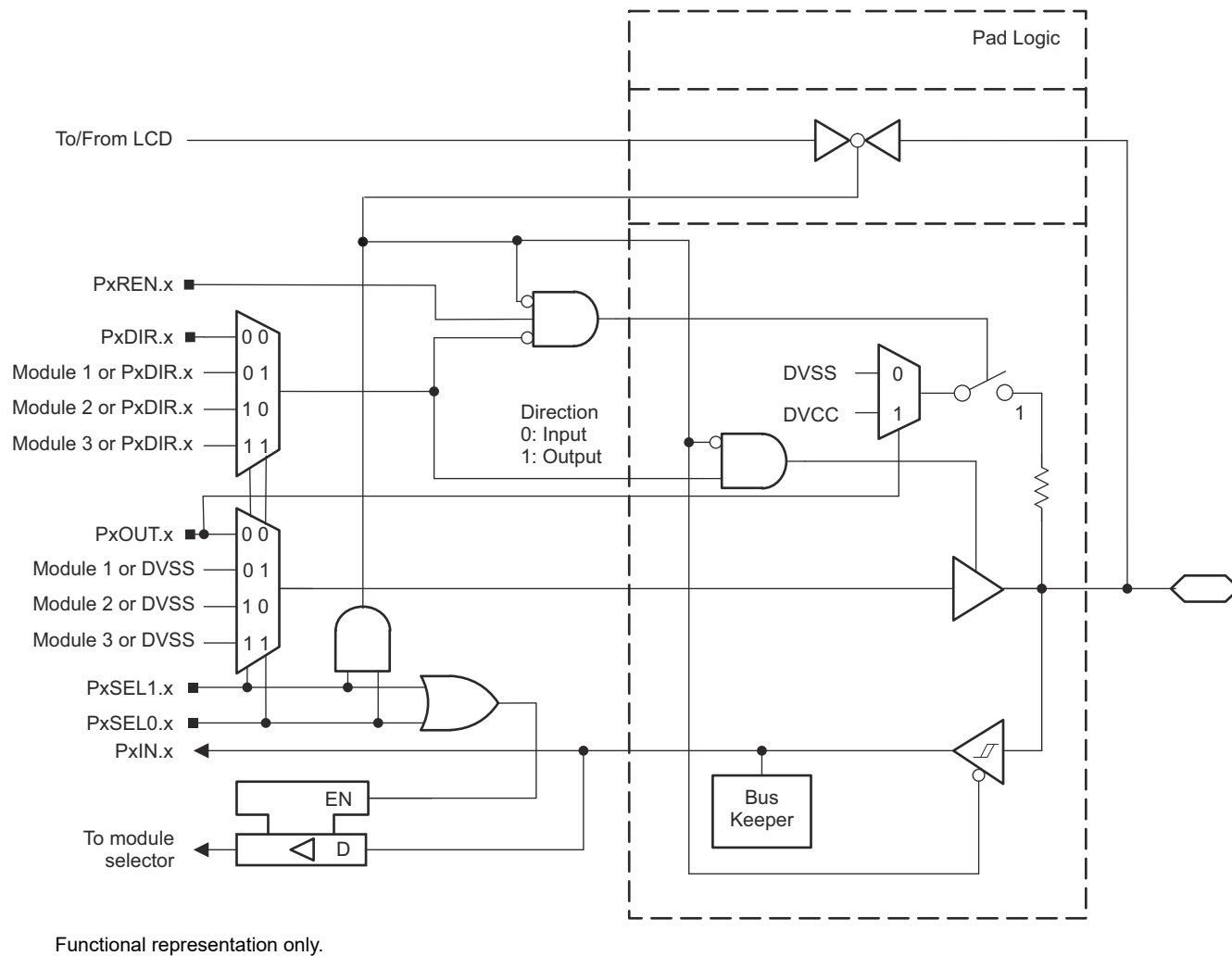
Figure 9-22. Port P6 (P6.4) Diagram
