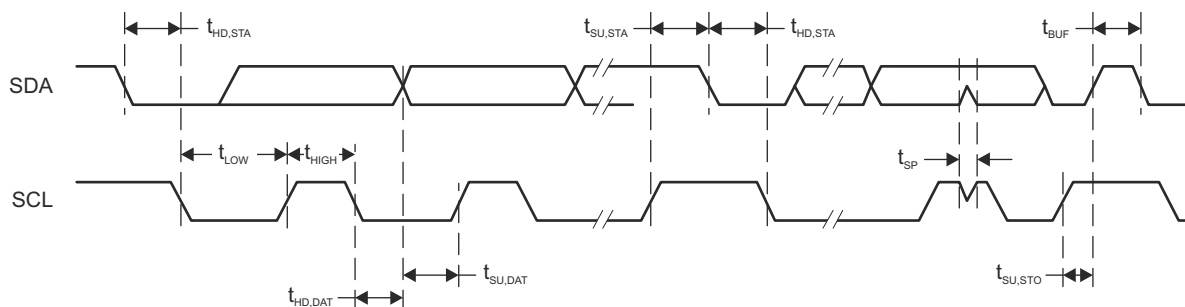
Figure 8-17. I 2 C Mode Timing
