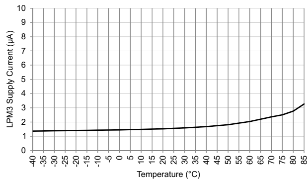
Figure 8-1. Low-Power Mode 3 Supply Current vs Temperature
