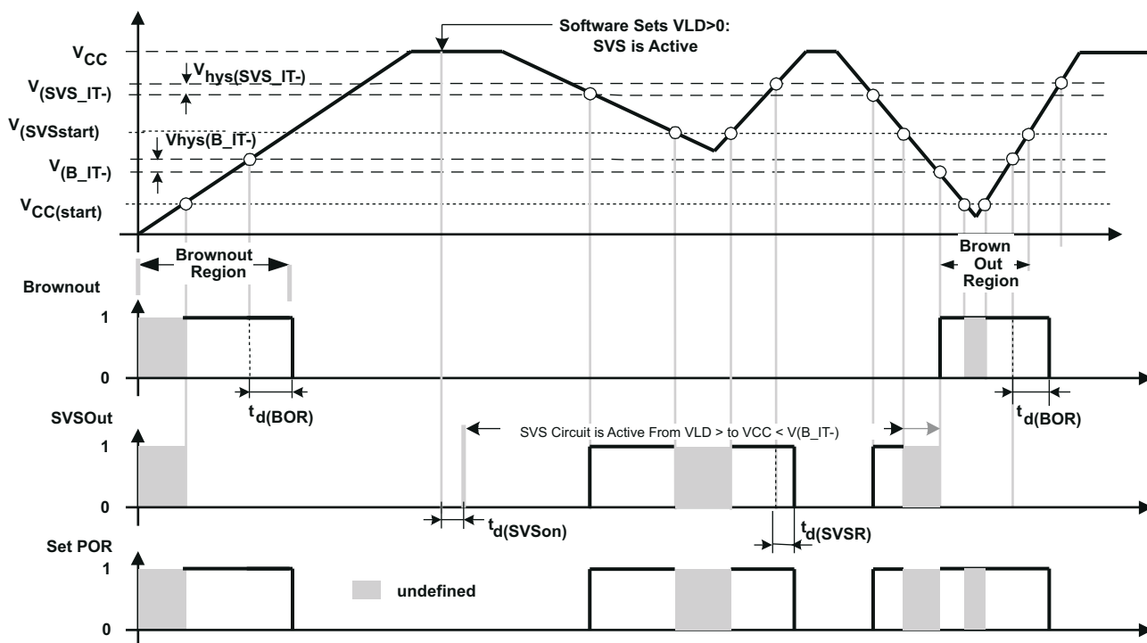
Figure 8-13. SVS Reset (SVSR) vs Supply Voltage
