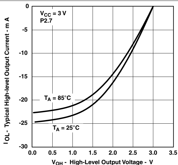
Figure 8-5. Typical High-Level Output Current vs Typical High-Level Output Current
