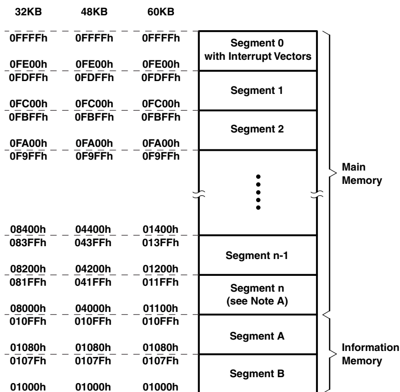
Figure 9-7. Flash Memory Segments
