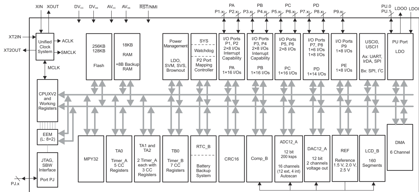
Figure 4-1. Functional Block Diagram – MSP430F6438, MSP430F6436
