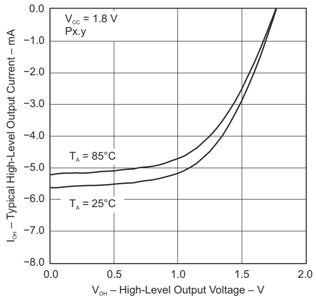
Figure 8-7. Typical High-Level Output Current vs High-Level Output Voltage
