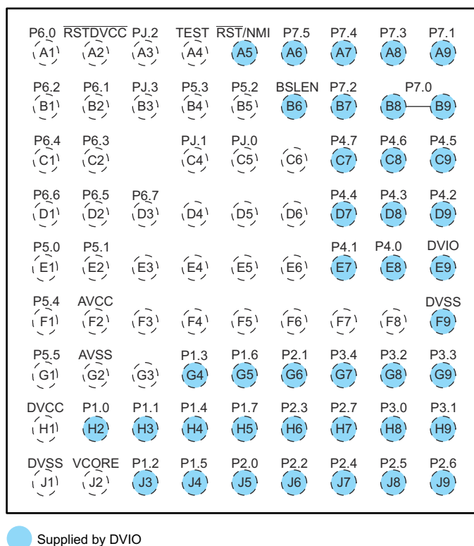
Figure 7-2. 80-Pin ZXH or ZQE Package (Top View)
