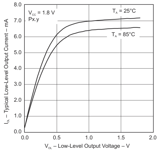
Figure 8-5. Typical Low-Level Output Current vs Low-Level Output Voltage
