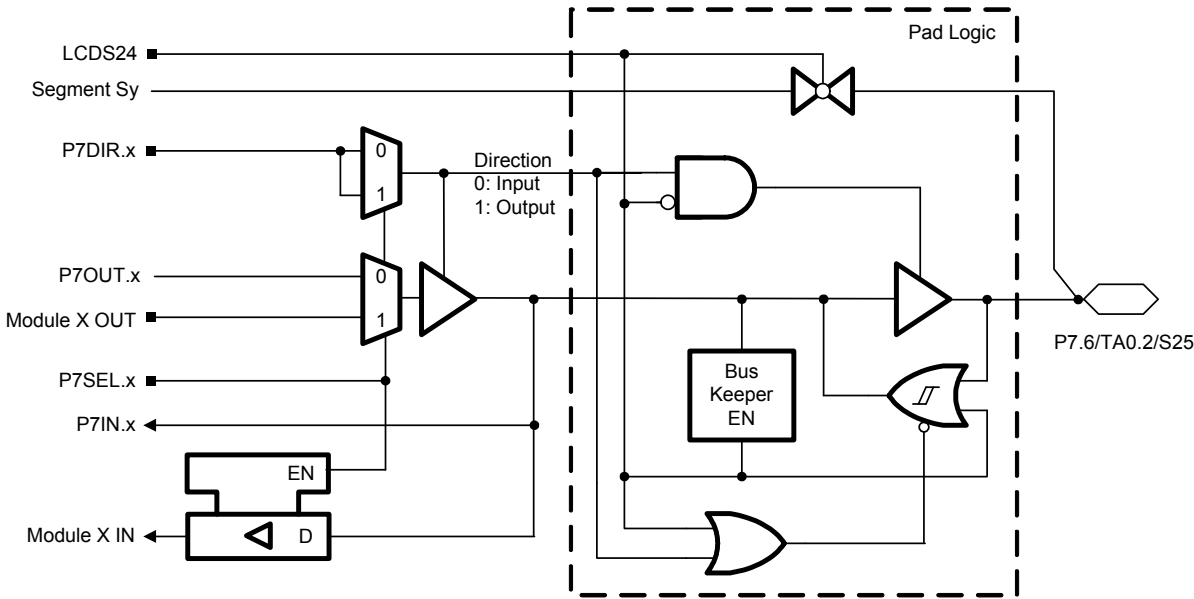
Port P7 (P7.6) pin functions
