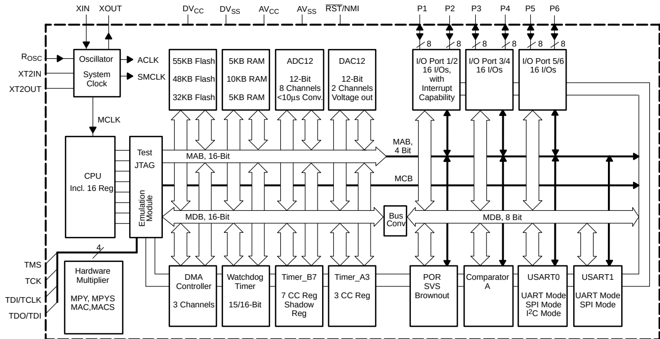
functional block diagram, MSP430F161x
