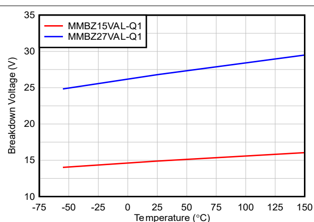
Figure 5-2. Breakdown Voltage vs Temperature
