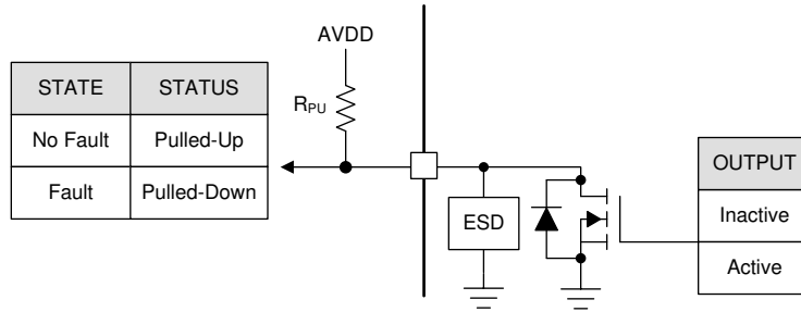
Figure 8-26. Open Drain
