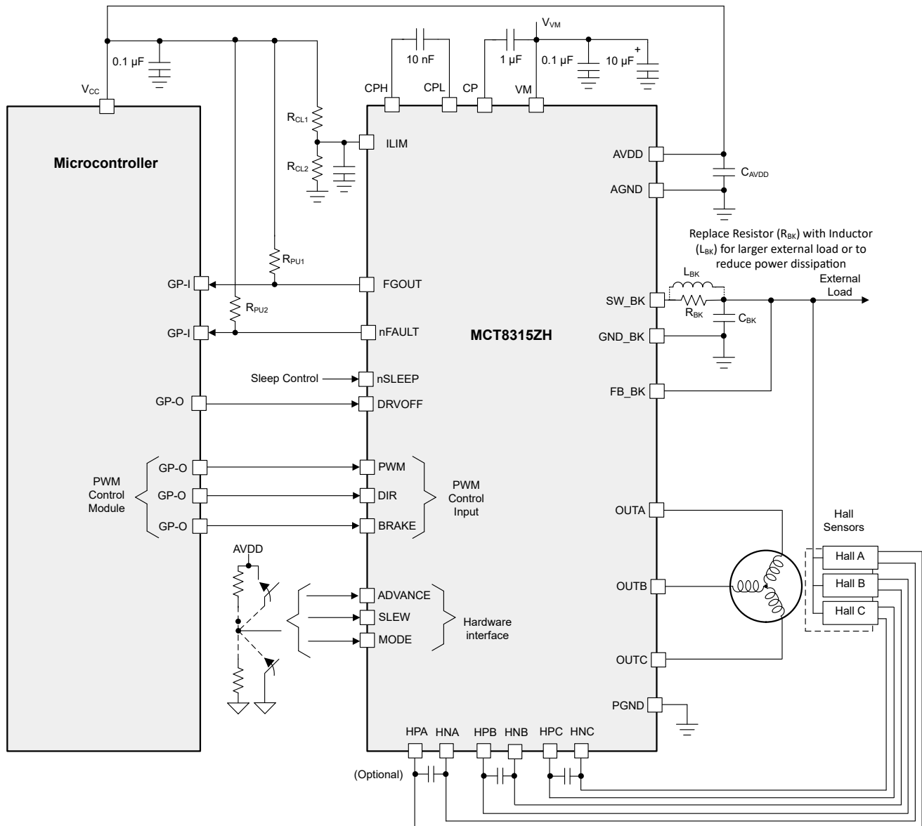
Figure 9-1. Primary Application Schematics for MCT8315ZH (hardware variant with buck)
