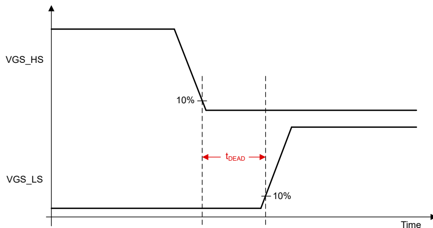
Figure 8-20. Dead Time
