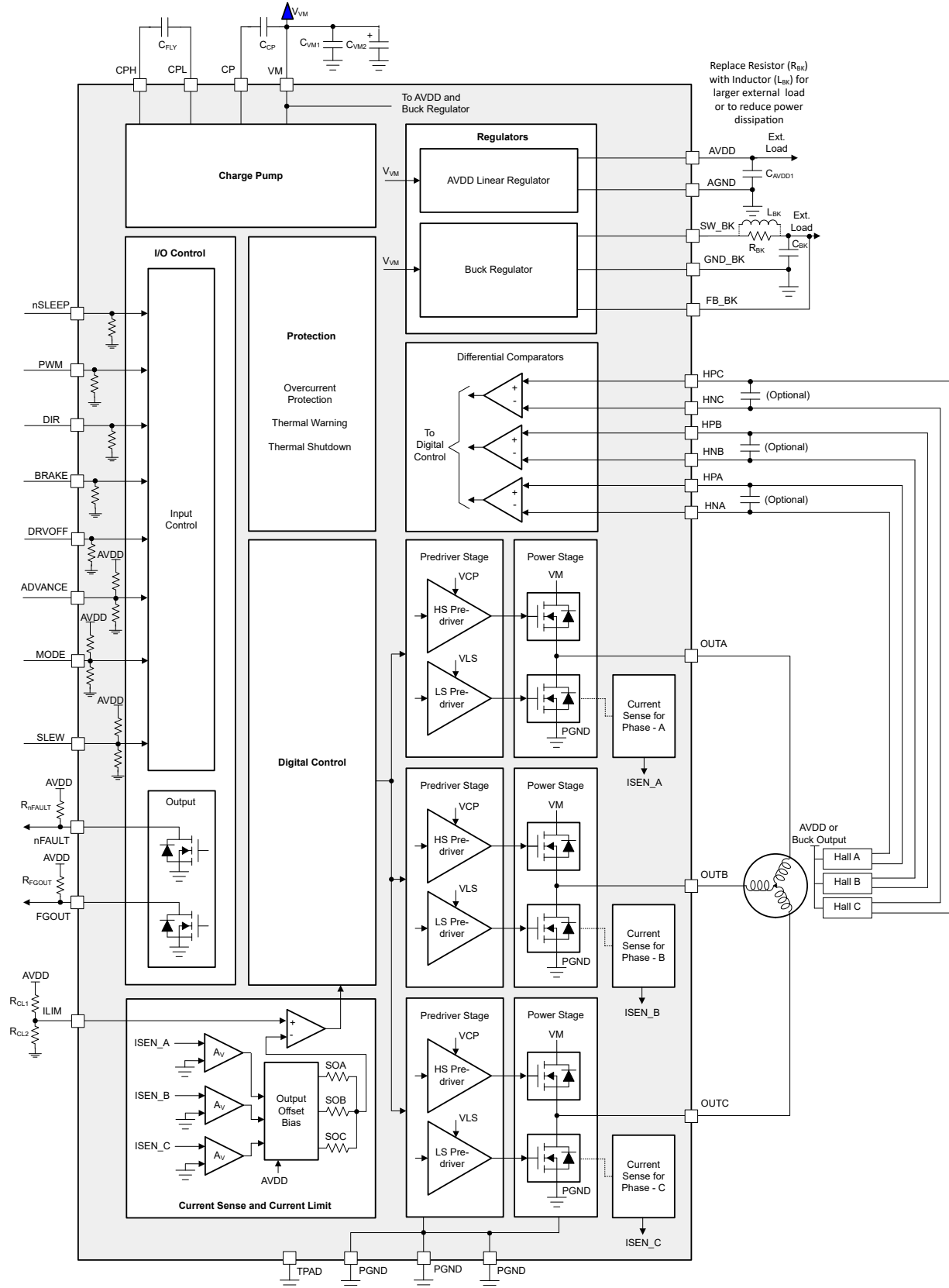
Figure 8-2. MCT8315ZH Block Diagram
