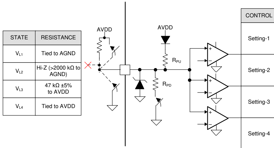
Figure 8-28. Four Level Input Pin Structure
