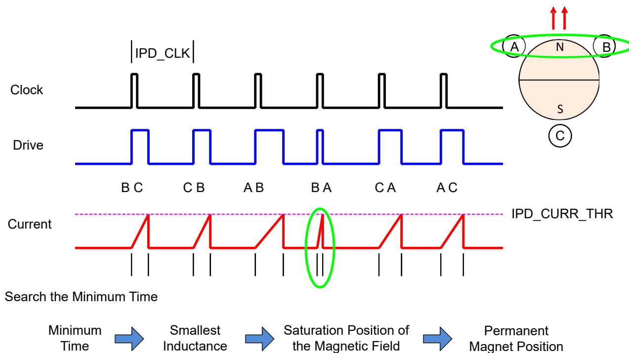
Figure 7-25. IPD Function
