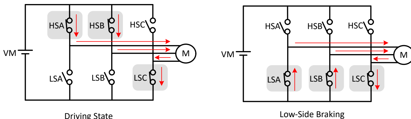
Figure 7-44. Low-Side Braking
