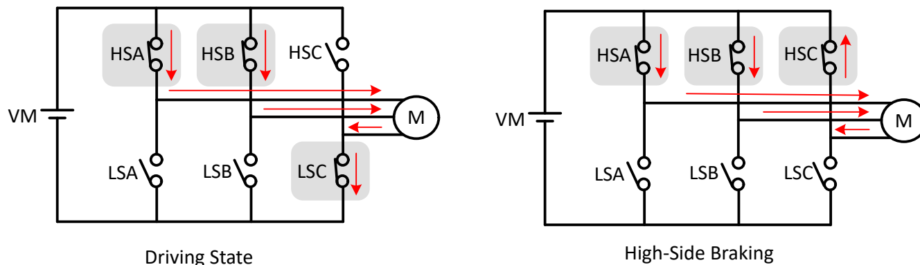
Figure 7-44. High-Side Braking
