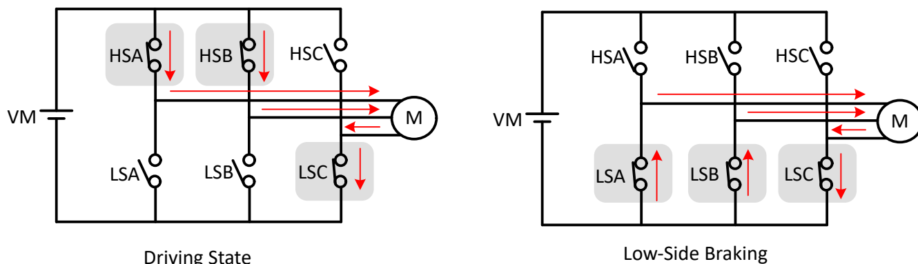
Figure 7-43. Low-Side Braking
