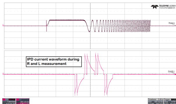
Figure 8-4. IPD current waveform during Rand L measurement
