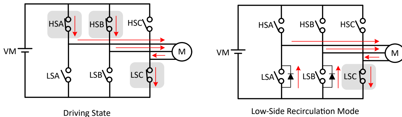
Figure 7-41. Low-Side Recirculation
