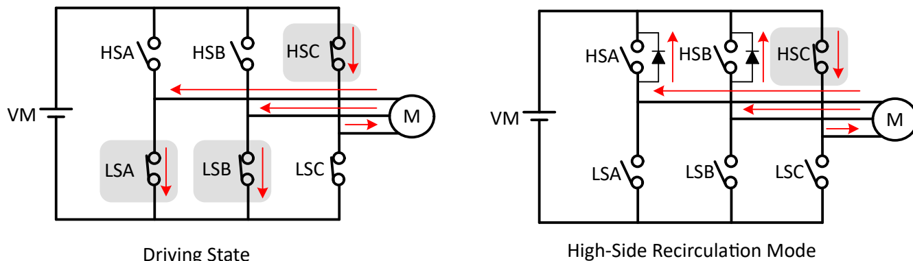
Figure 7-42. High-Side Recirculation
