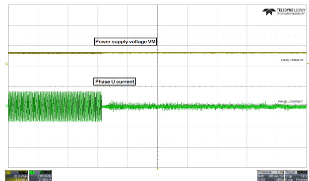
Figure 8-10. Power supply voltage and phase current waveform when AVS is enabled
