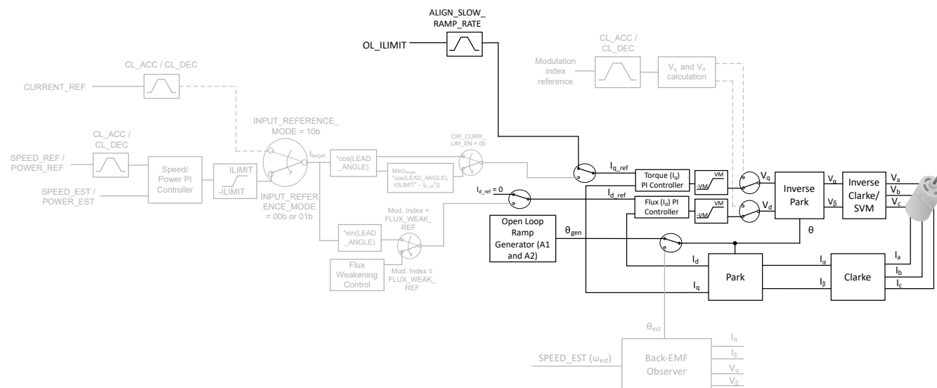
Figure 6-37. Open Loop
