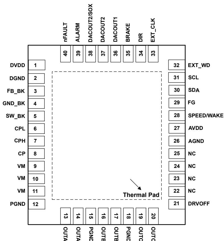
Figure 4-1. MCF8315C-Q1, 40-Pin RGF VQFN With Exposed Thermal Pad, Top View
