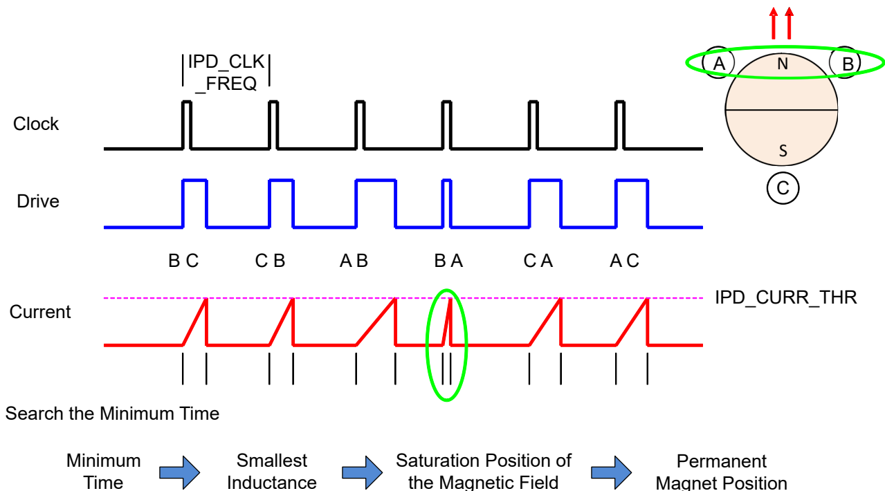
Figure 6-26. IPD Operation
