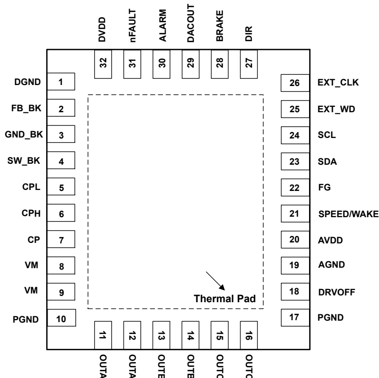
Figure 4-2. MCF8315C-Q1, 32-Pin RRY WQFN With Exposed Thermal Pad, Top View
