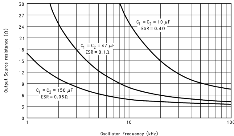
Figure 15. Output Source Resistance vs Oscillator Frequency
