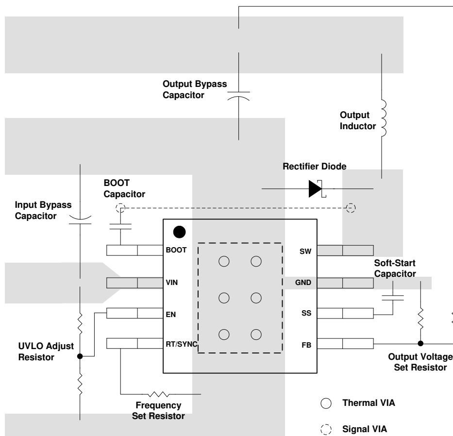
Figure 7-10. Layout
