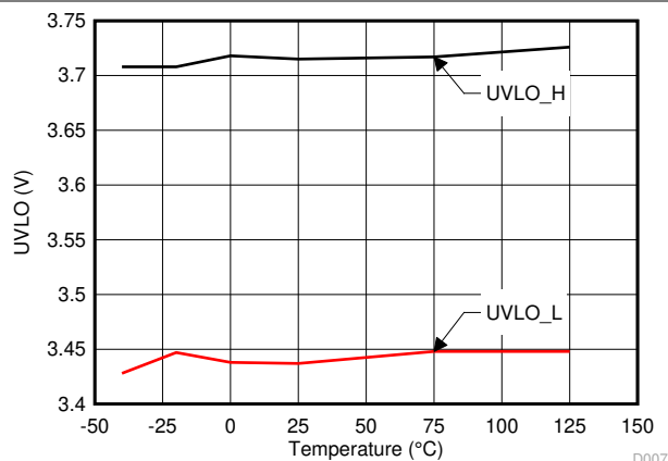
Figure 5-12. UVLO Threshold
