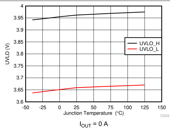
Figure 7-10. UVLO Threshold
