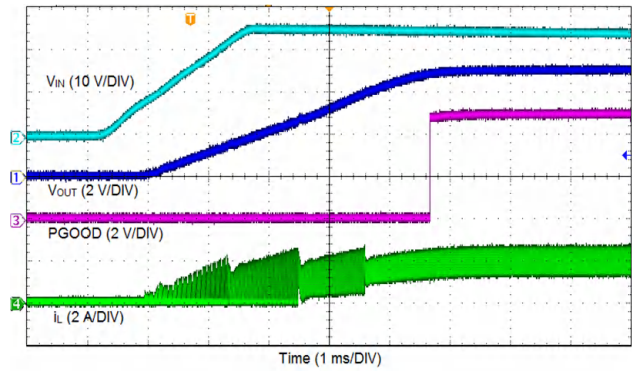
Figure 9-3. Start-up By V_{IN}
