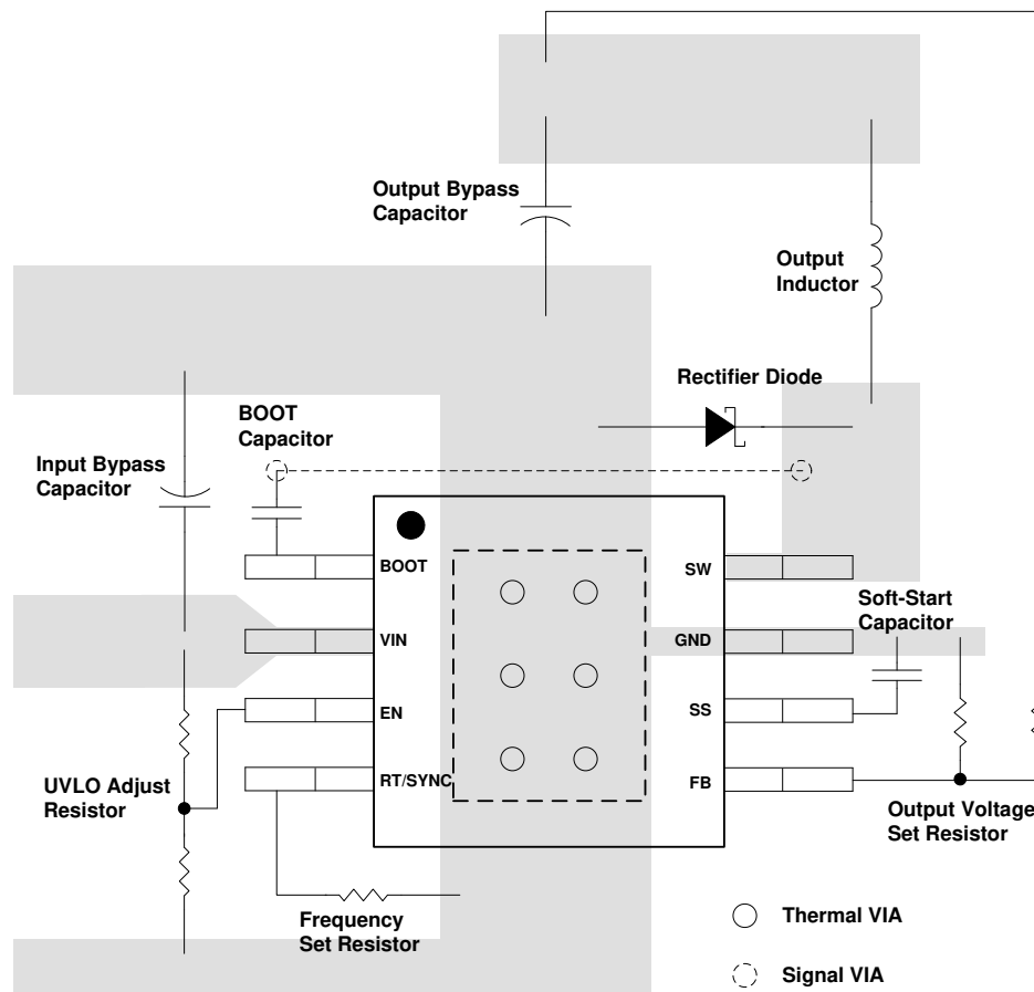
Figure 11-1. Layout
