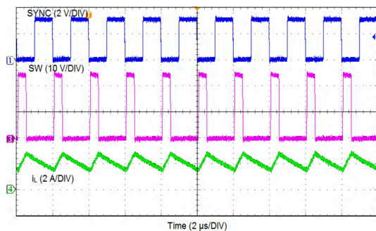
Figure 8-6. Synchronizing in CCM
