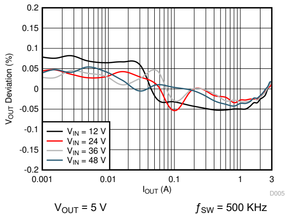
Figure 7-5. Load Regulation
