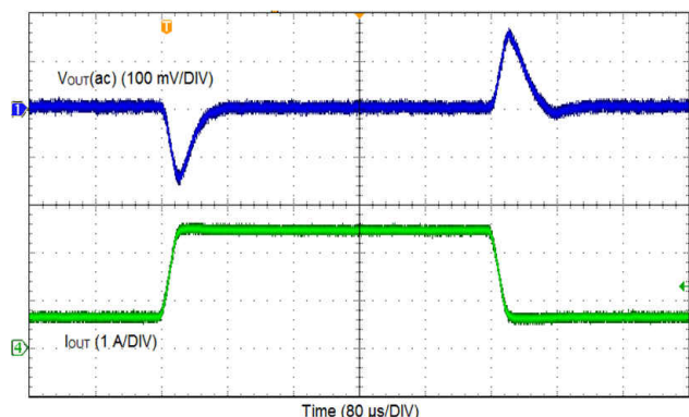
Figure 9-5. DCM Mode
