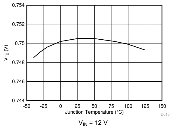
Figure 7-8. Voltage Reference vs Junction Temperature
