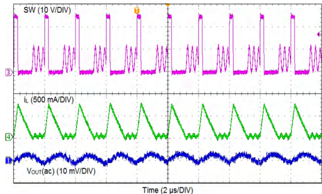
Figure 9-5. DCM Mode
