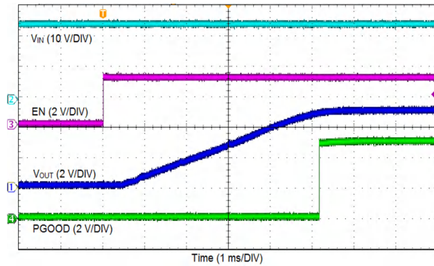
Figure 9-2. Start-up by EN
