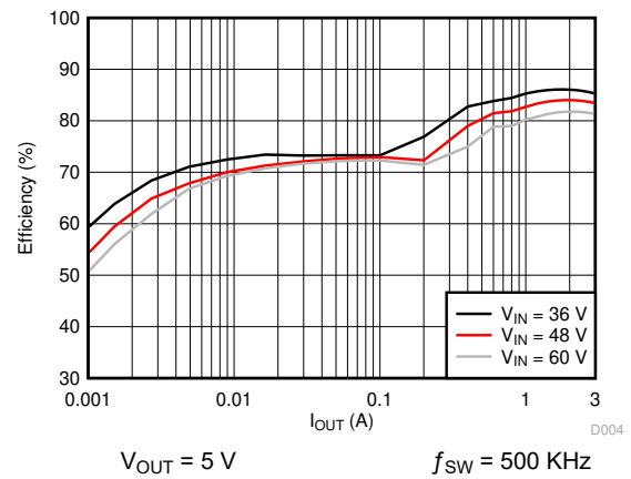
Figure 7-4. Efficiency vs Load Current
