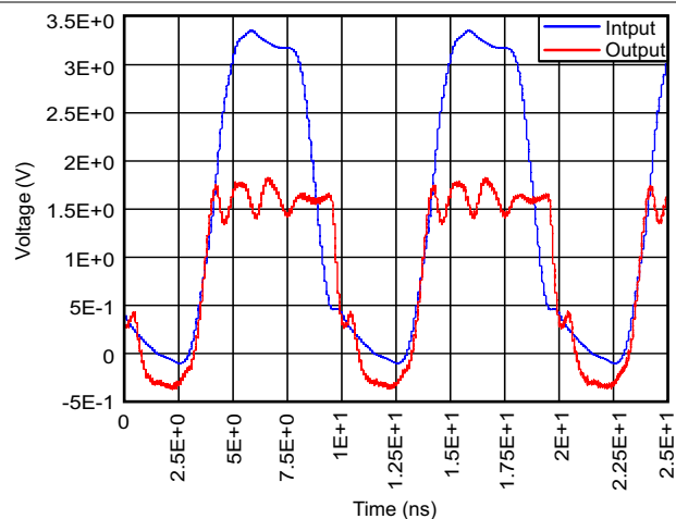
Figure 12-3. Waveform From TP1 (Pullup Resistor: 160- \Omega and 50-pF Capacitance 3.3 to 1.8 V at 100 MHz)
