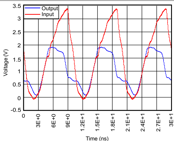
Figure 12-4. Waveform From TP2 (Pullup Resistor: 160- \Omega and 50-pF Capacitance 1.8 to 3.3 V at 100 MHz)
