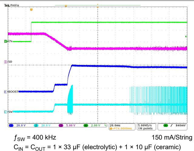
Figure 8-4. Typical Start-Up
