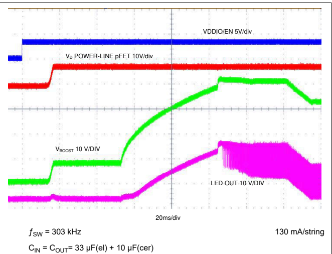
Figure 7-5. Typical Start-up
