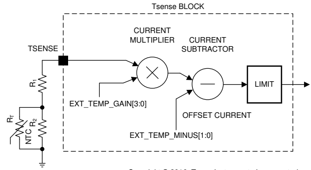
Figure 6-28. NTC Current Processing — Scaling, Shift, and Limitation
