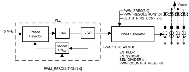
Figure 6-3. PWM Clcking With PLL, Internal Oscillator as Reference
