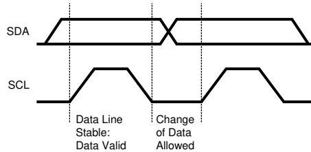
Figure 6-39. Bit Transfer
