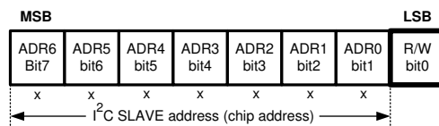
Figure 6-42. Address and Read/Write Bit
