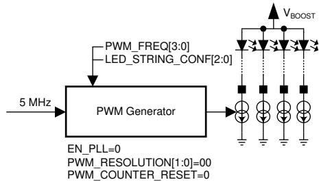
Figure 6-2. PWM Clcking With Internal Oscillator
