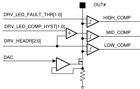
Figure 6-20. Output Voltage Comparators
