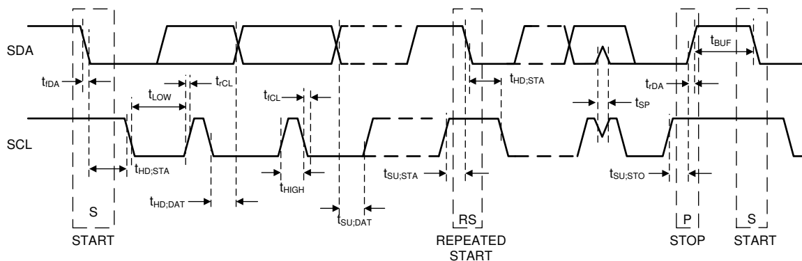
Figure 7-17. I²C-Compatible Timing
