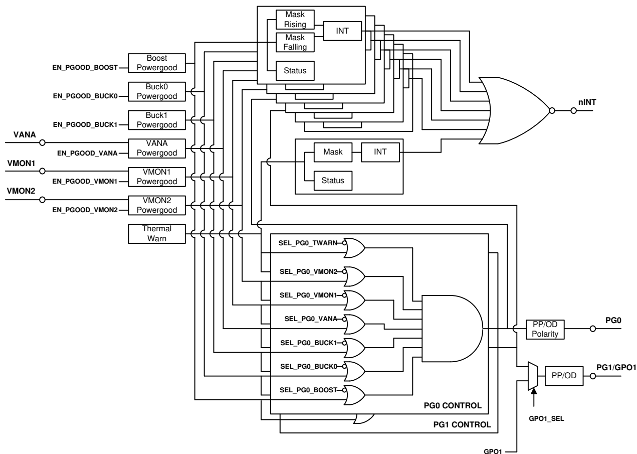
Figure 7-9. Block Diagram of Power-Good Connections
