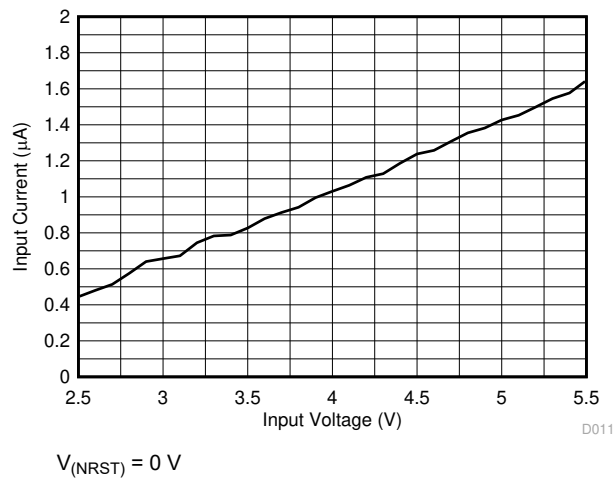
Figure 6-2. Shutdown Current Consumption vs Input Voltage
