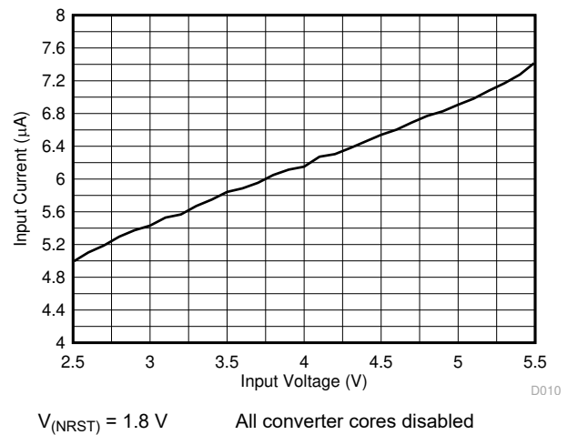
Figure 6-3. Standby Current Consumption vs Input Voltage
