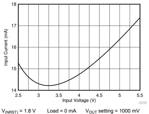
Figure 6-5. PWM Mode Current Consumption vs Input Voltage —One Output Enabled
