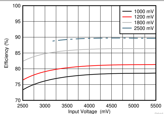
Figure 8-3. Efficiency vs Input Voltage in PFM Mode
