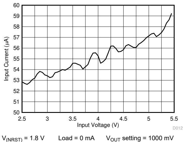
Figure 6-4. PFM Mode Current Consumption vs Input Voltage —One Output Enabled
