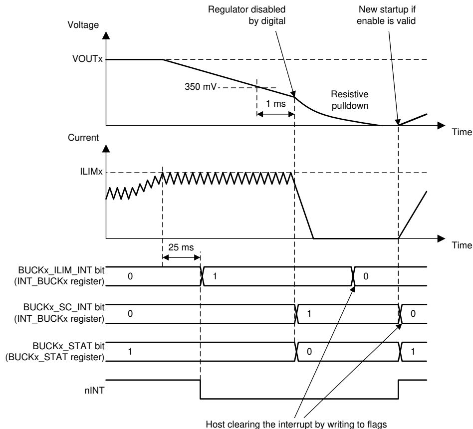
Figure 7-6. Overload Situation
