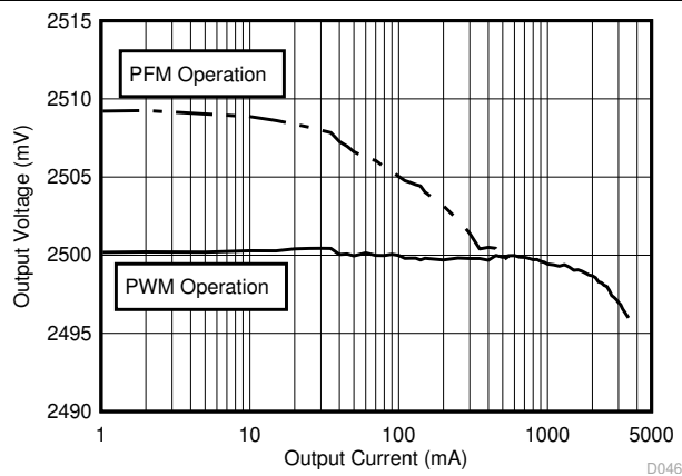
Figure 8-6. DC Load Regulation in PWM mode
