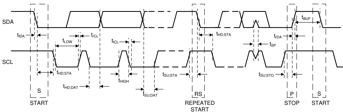
Figure 6-1. I²C Timing
