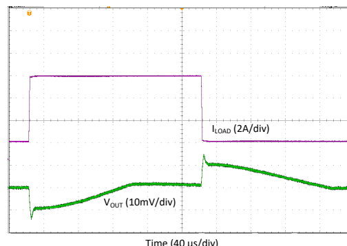
Figure 8-13. Transient Load Step Response, Forced-PWM-Four-Phase Mode, T_A = +125^\circ\text{C}
