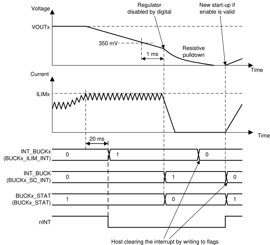
Figure 7-10. Overload Situation
