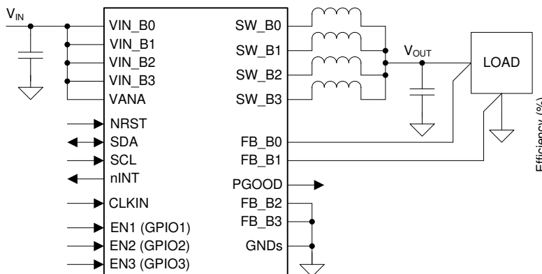
Simplified Schematic
