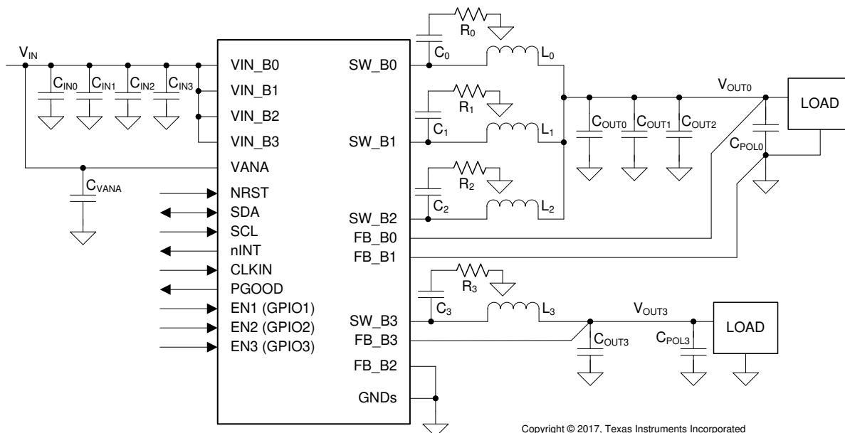
Figure 29. 3-Phase and 1-Phase Configuration (LP87562-Q1)
