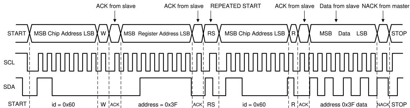
Figure 26. Read Cycle ( r = \text{read} ; \text{SDA} = 1 ), Using Example \text{id} = \text{Device Address} = 0x60 for LP8756x-Q1
