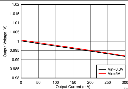
Figure 8-21. LDO Output Voltage vs Load Current
