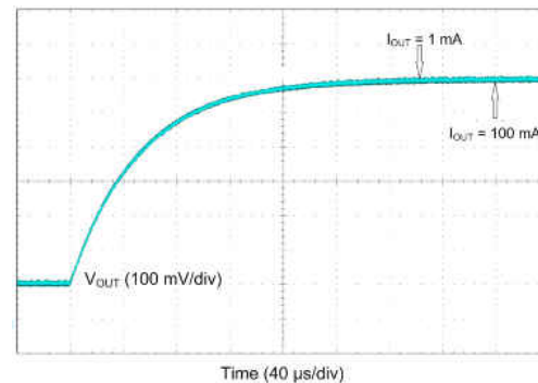
Figure 8-29. LDO V_{OUT} Transition from 1.2 V to 1.8 V
