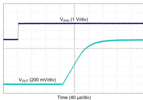
Figure 8-45. LDO Start-Up
