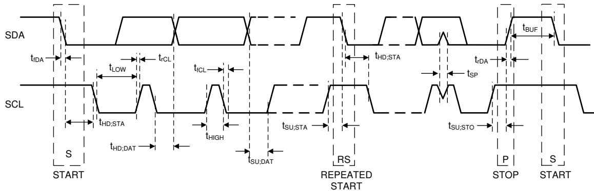
Figure 7-16. I²C-Compatible Timing
