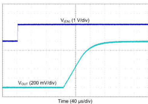
Figure 8-24. LDO Start-Up
