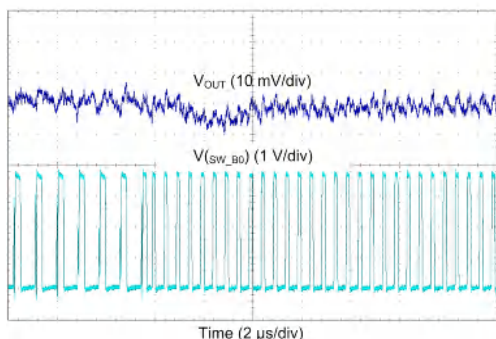
Figure 8-14. Buck Transient From PFM-to-PWM Mode
