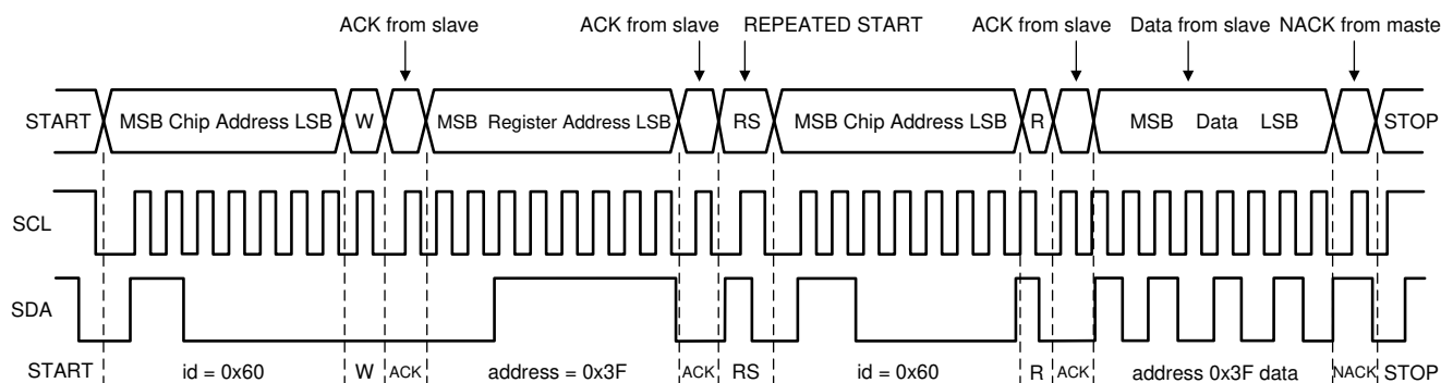
Figure 7-18. Read Cycle (r = read; SDA = 1). Example Device Address = 0x60
