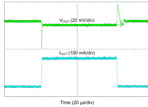
Figure 8-27. LDO Transient Load Step Response
