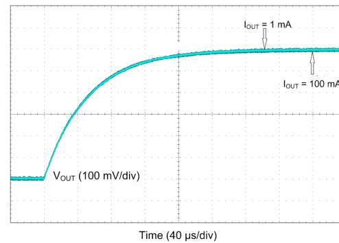
Figure 8-29. LDO V_{OUT} Transition from 1.2 V to 1.8 V
