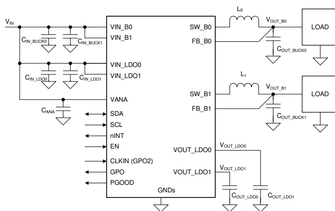
Figure 8-1. LP873222-Q1 Typical Application
