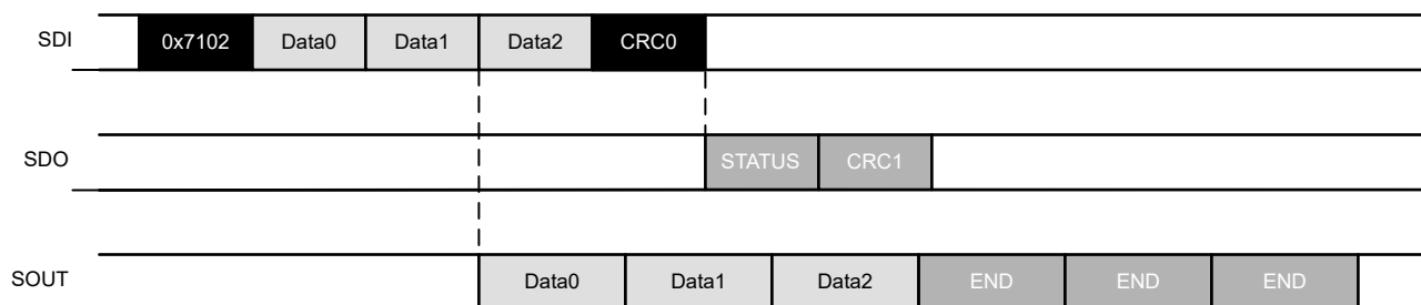
Figure 7-15. Example of FWD_RD_END command
