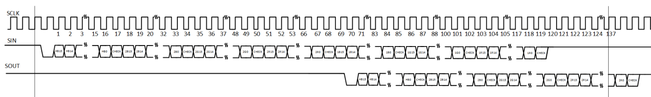
Figure 8-20. Data Write Command with Non-Broadcast (Timing Diagram)
