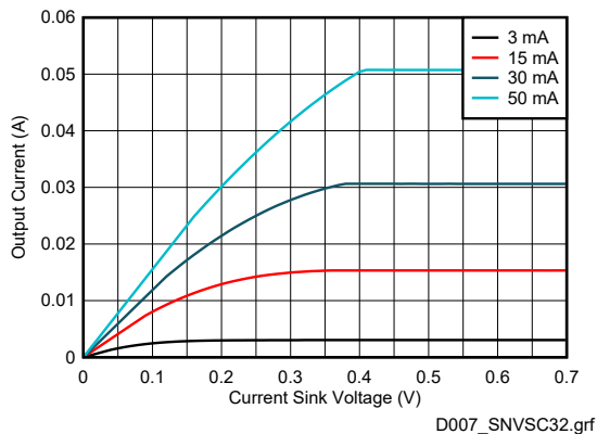
Figure 7-7. Current Sinks Voltage vs Current
