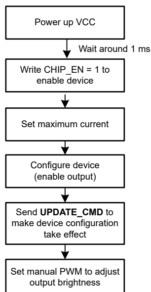
Figure 8-2. Program Procedure
