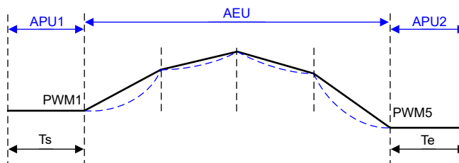
Figure 7-20. APU example
