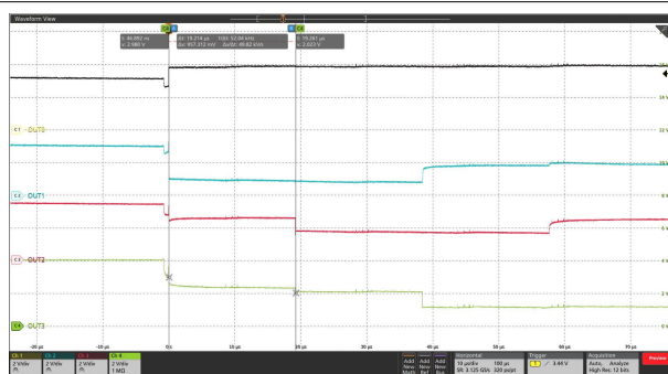
Figure 8-4. PWM Alignment Enabled
