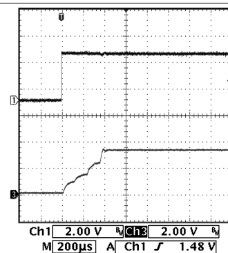
Figure 25. Line Transient Response
