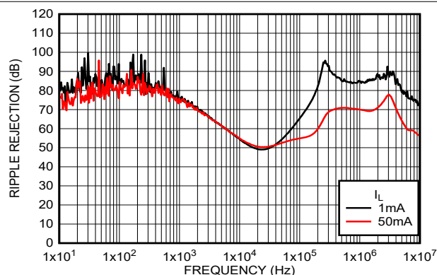
Figure 5-28. Ripple Rejection (Legacy Chip)
