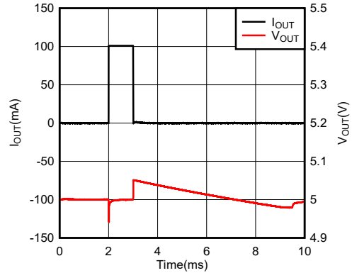
Figure 5-48. Load Transient Response vs Time (New Chip)
