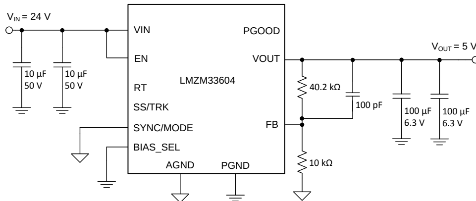
Figure 45. LMZM33604 Typical Schematic
