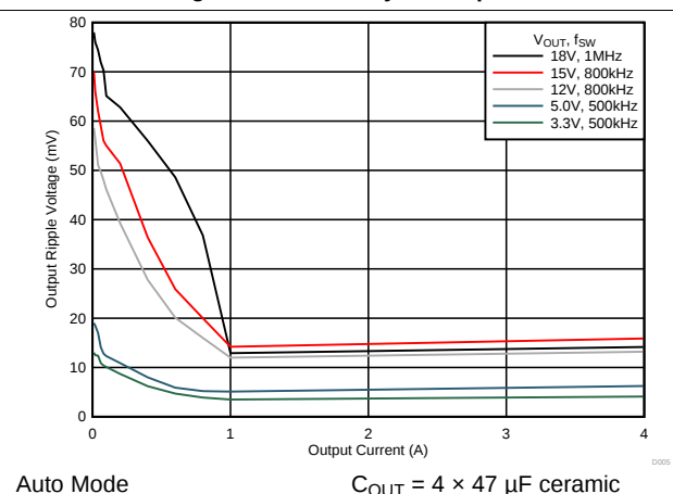
Figure 16. Output Voltage Ripple
