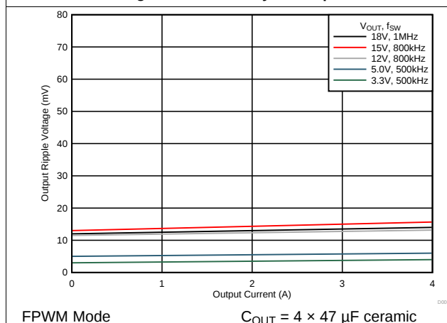
Figure 15. Output Voltage Ripple
