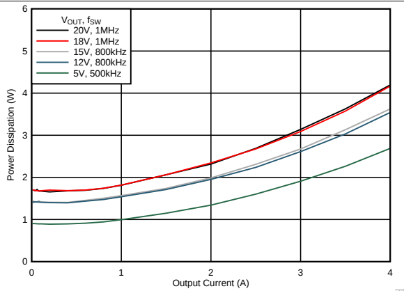
Figure 27. Power Dissipation
