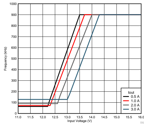
Figure 23. Frequency Foldback
