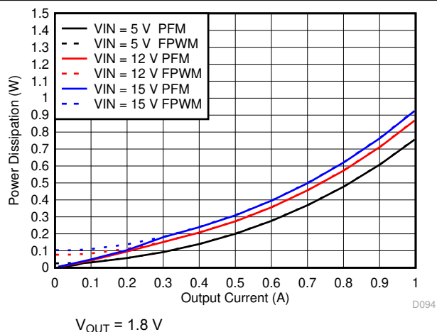
Figure 6-15. Power Dissipation
