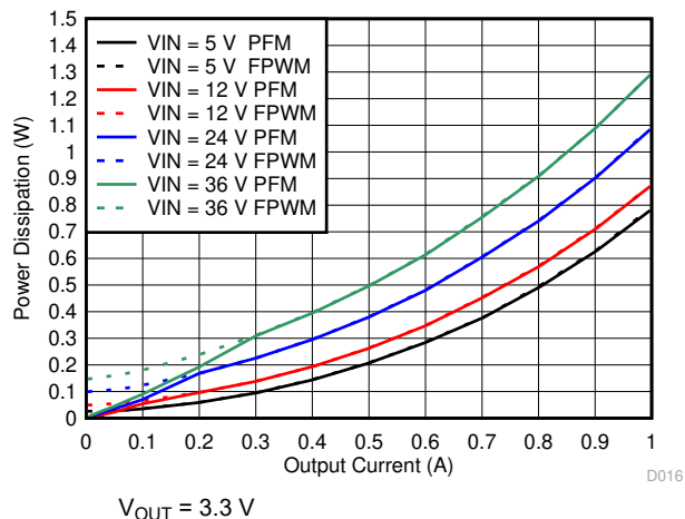
Figure 6-13. Power Dissipation
