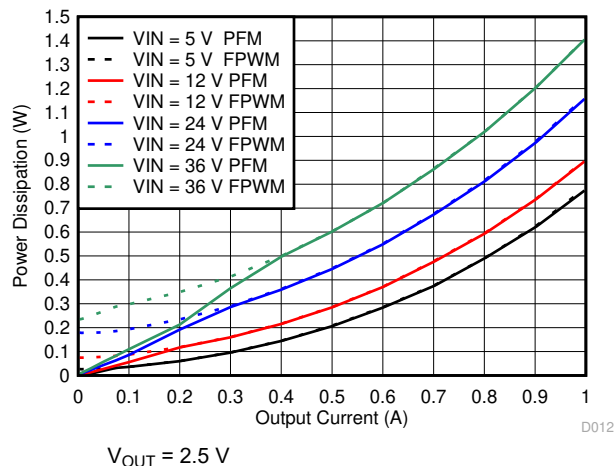
Figure 6-14. Power Dissipation
