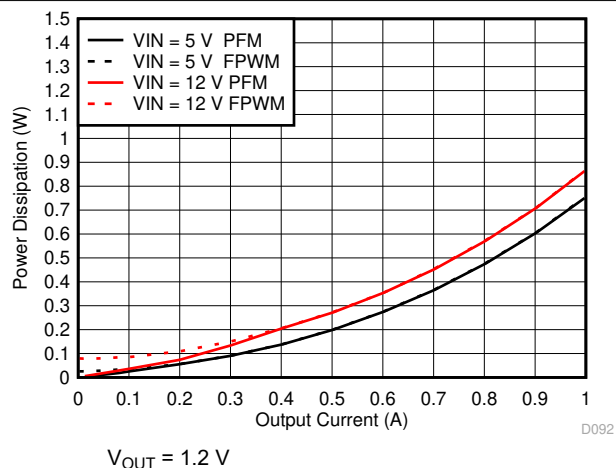
Figure 6-16. Power Dissipation
