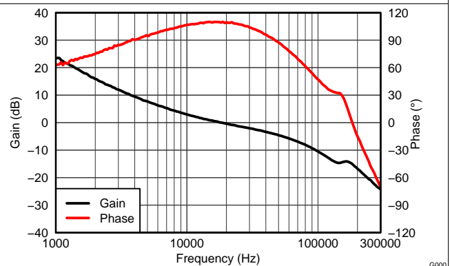
Figure 18. V OUT = 12 V, I OUT = 2 A, C OUT1 = 44 µF ceramic, C OUT2 = 56 µF electrolytic, f SW = 800 kHz
