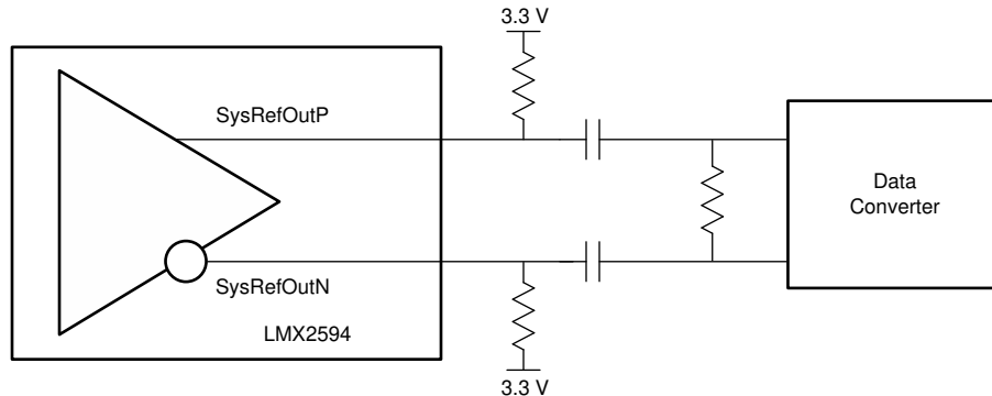
Figure 28. SYSREF Output
