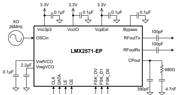
Figure 8-12. Typical Synthesizer Duplex Mode Application Schematic
